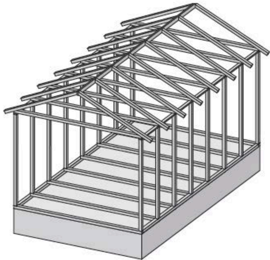
Fig. 14-26 Wood-frame construction.
