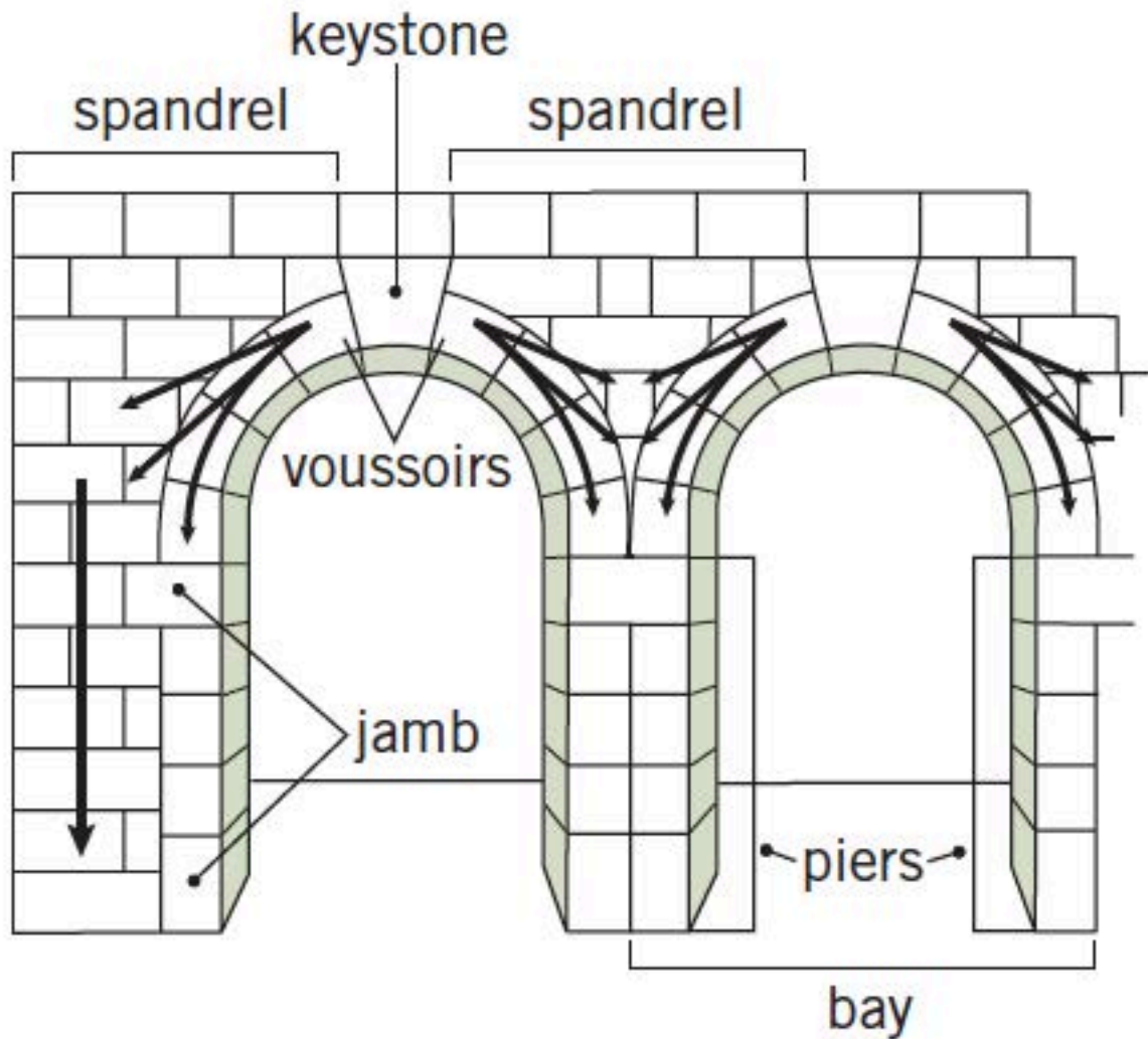
Fig. 14-12 Round arch.
