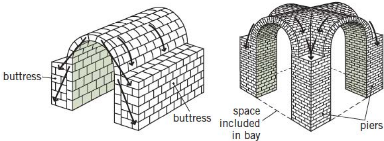
Fig. 14-14 Barrel vault (left) and groin vault (right).
